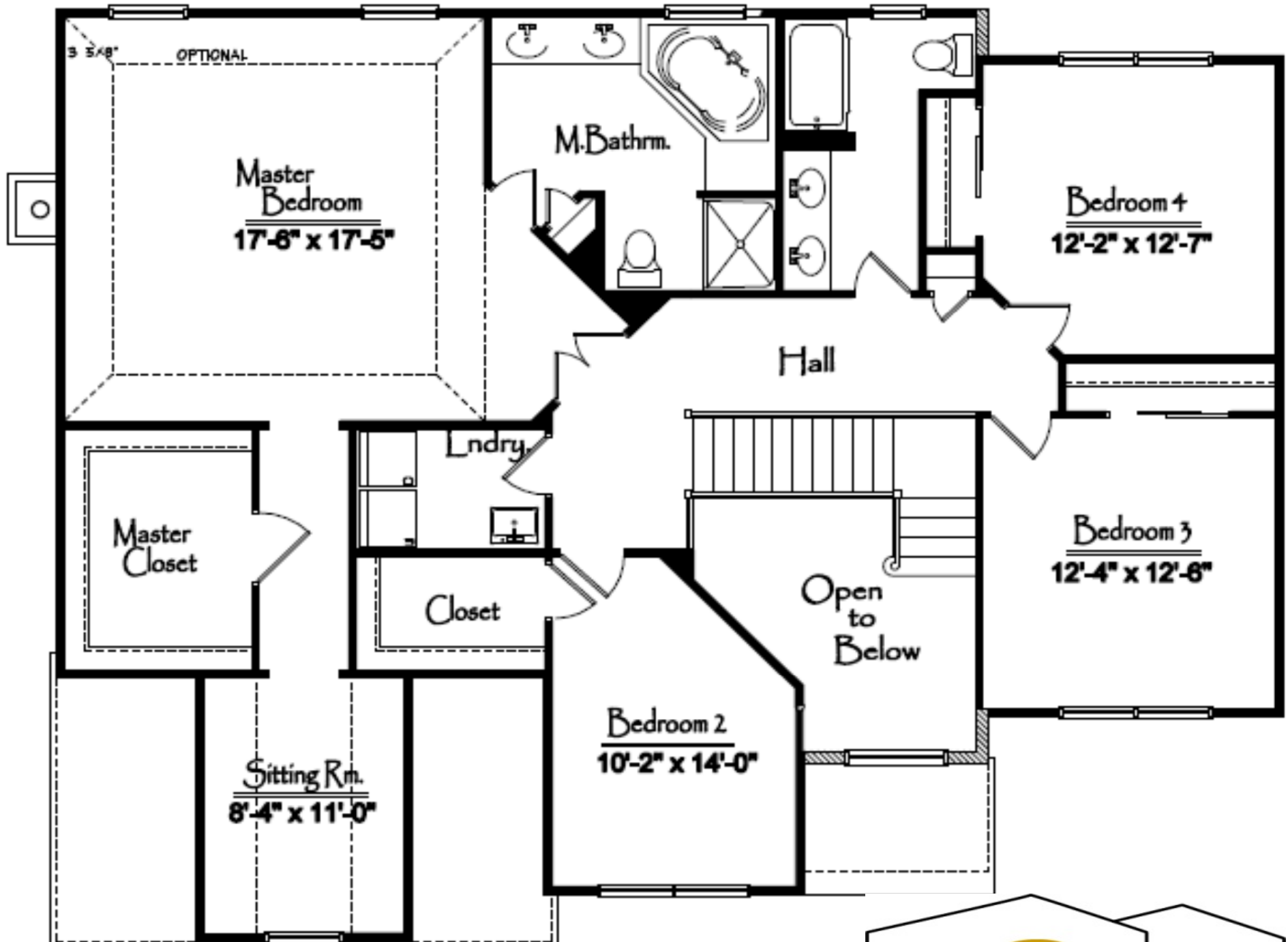
SUSSEX SECOND FLOOR 1,575 Square Feet
