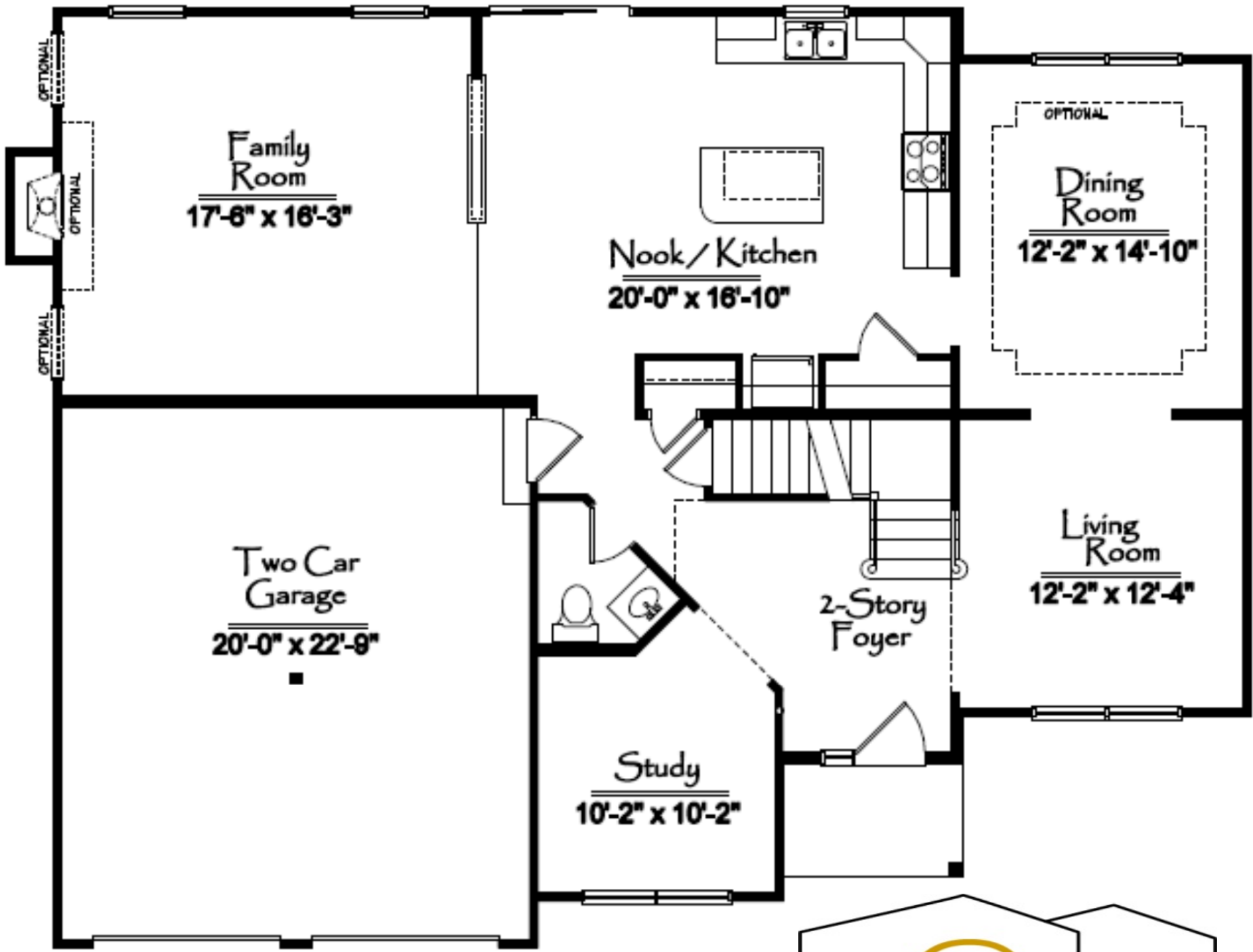
SUSSEX FIRST FLOOR 1,360 Square Feet
